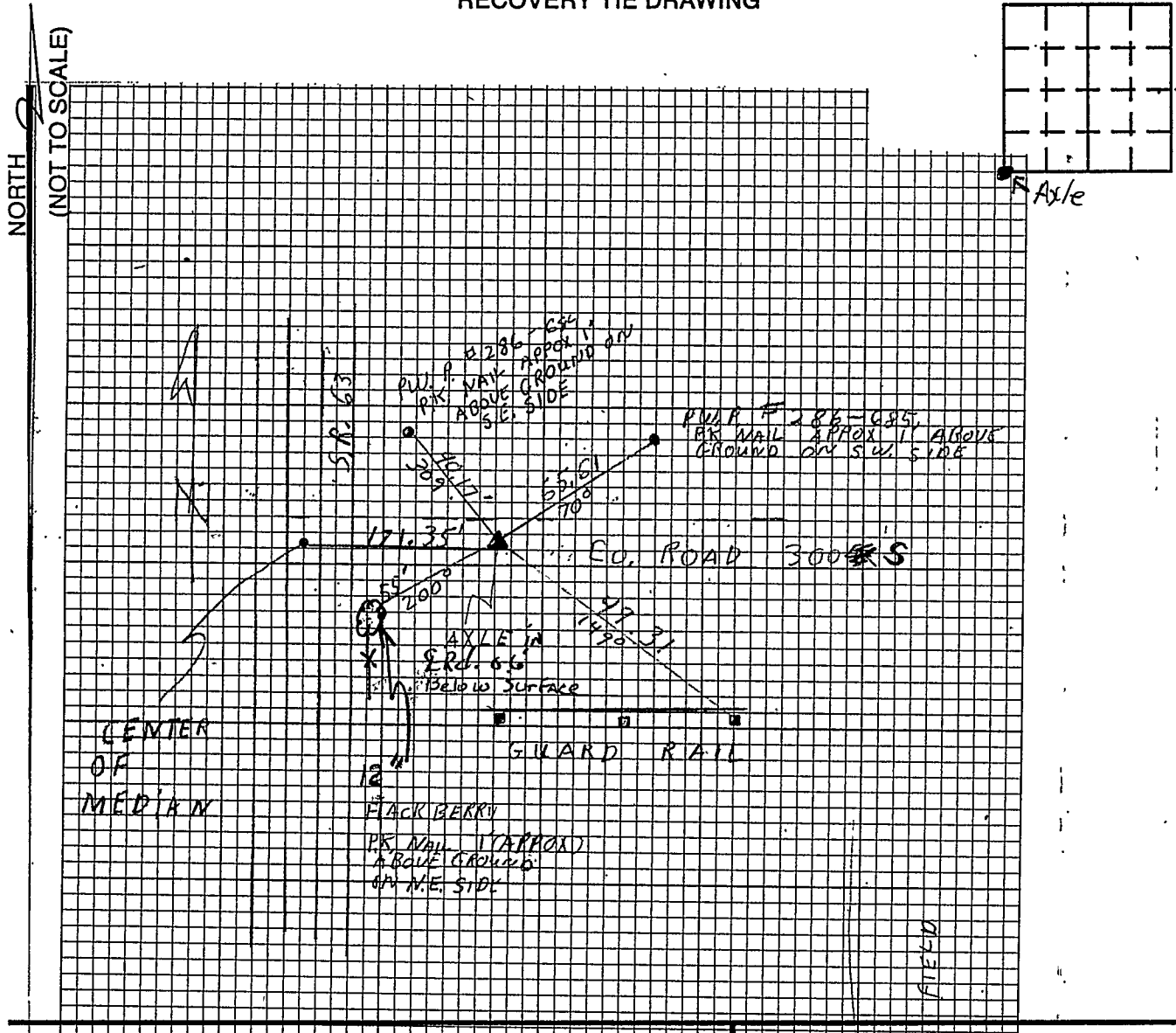
RECOVERY TIE DRAWING
