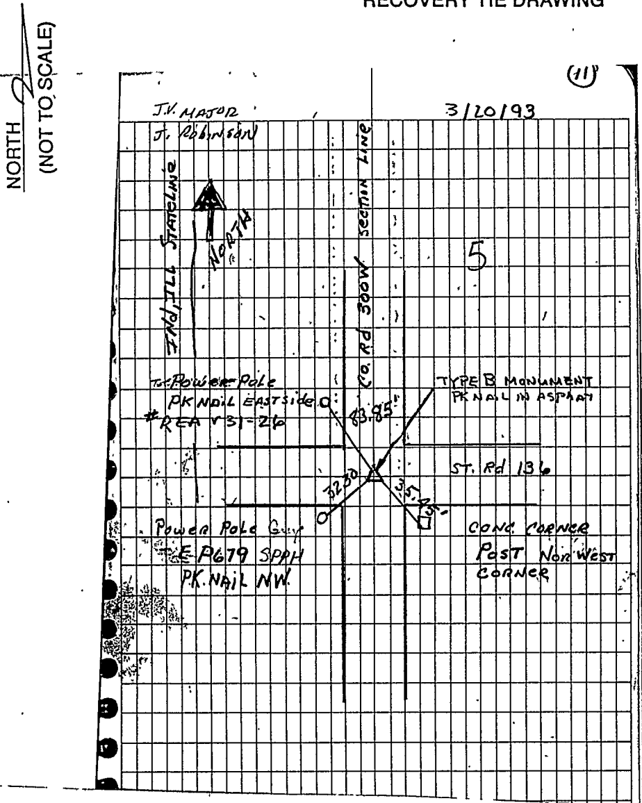
RECOVERY TIE DRAWING
